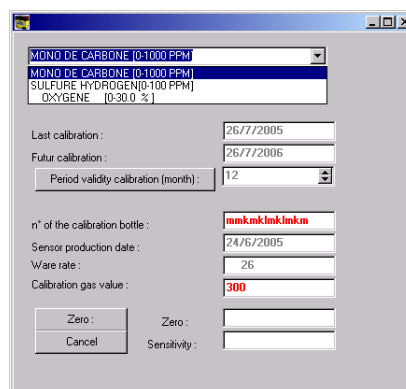
Figure 41: Calibration menu
