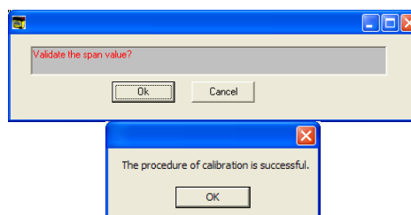
Figure 42: confirming Calibration
